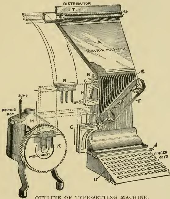
OUTLINE OF TYPE-SETTING MACHINE.
